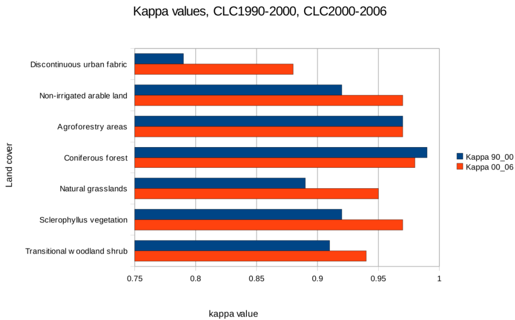
[Figure 6: kappa index of agreement across 7 largest land cover categories, 2000-2006]
